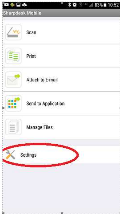
Select "Settings"
